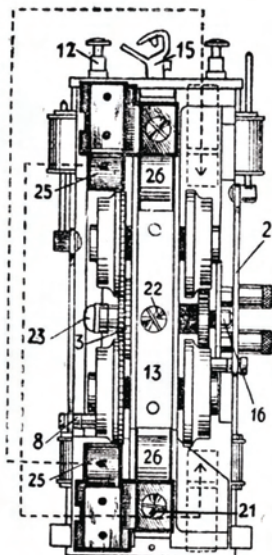
NOTE.—Diagrams show 0-4-0 mechanism. 4-4-0 mechanism is the same except that no outside shoes or front weight and spring are fitted.
